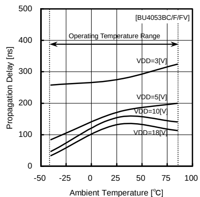
Fig.35 propagation delay time tPLZ (CONT—OUT)
