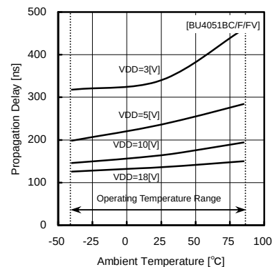
Fig.13 propagation delay time tPLZ (CONT – OUT)
