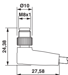
M8 x 1 male plug, angled version
