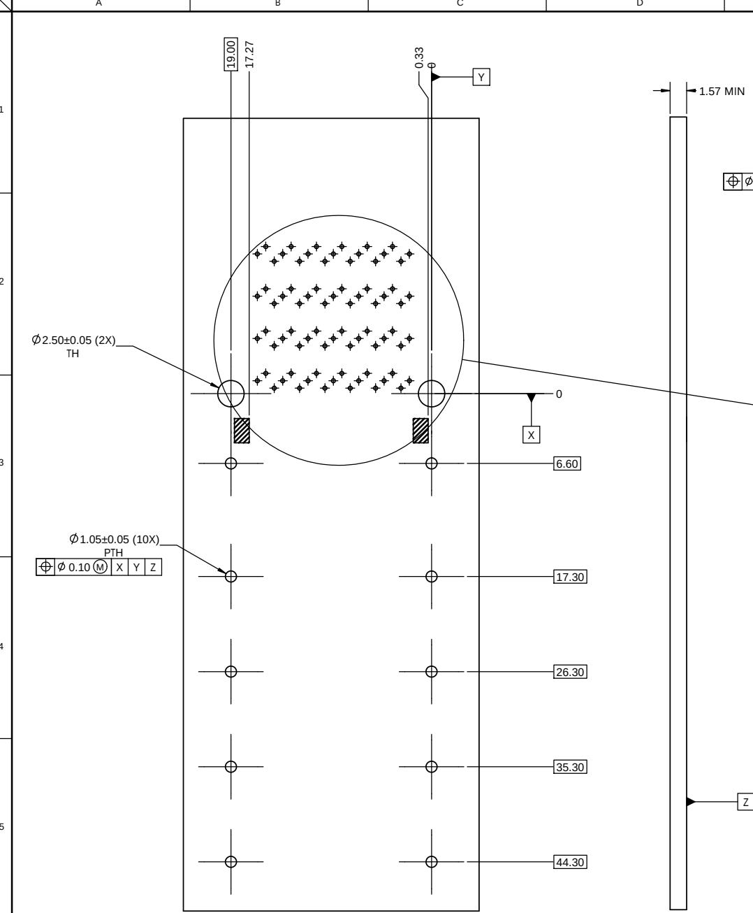
RECOMMENDED PCB BOARD LAYOUT COMPONENT SIDE SHOWN
