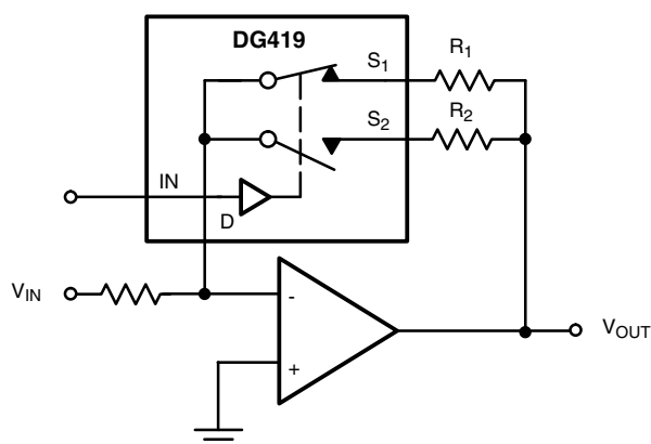
Figure 12. Programmable Gain Amplifier
