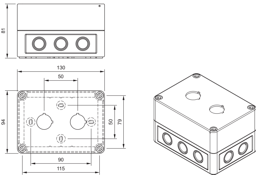
3 Stop pushbutton enclosure page 24
