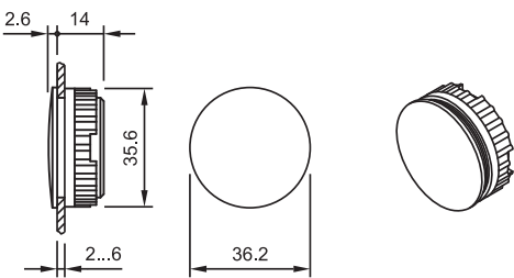
1 Blind plug page 16
