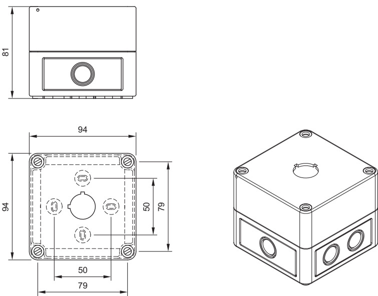
2 Stop pushbutton enclosure page 24
