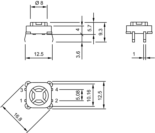
15 Switching element PCB mounting illuminative page 21
