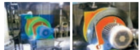
Alpha Blending
