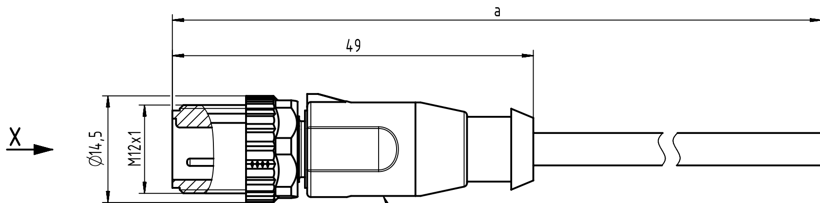
M12 A-coded 3-pole, male straight connector
