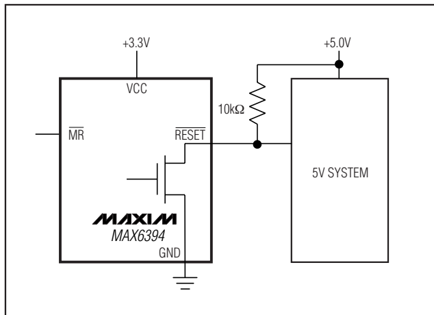
Figure 1. MAX6394 Open-Drain \overline{RESET} Output Allows Use with Multiple Supplies
