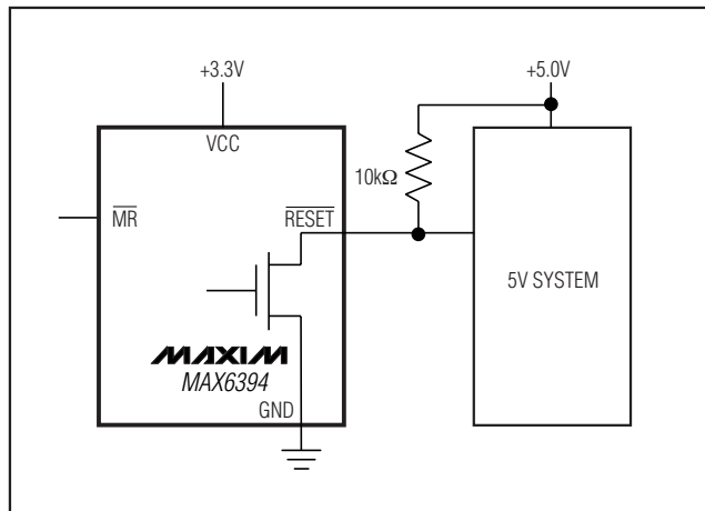
Figure 1. MAX6394 Open-Drain \overline{\text{RESET}} Output Allows Use with Multiple Supplies
