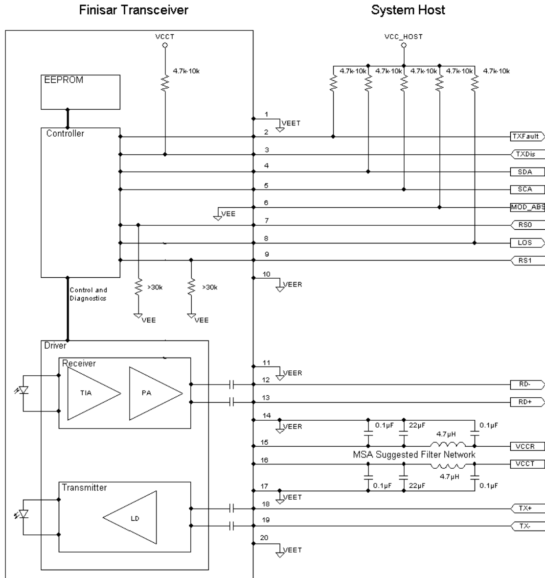
Figure 6-Host-Module Interface
