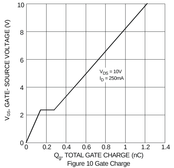
Figure 10 Gate Charge
