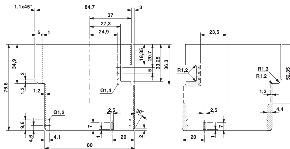
Dimensional drawing
