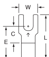
M10-8FB Stud Size 8 Wire Range 12-10
