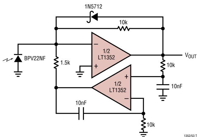
400kHz Photodiode Preamp with 10kHz Highpass Loop
