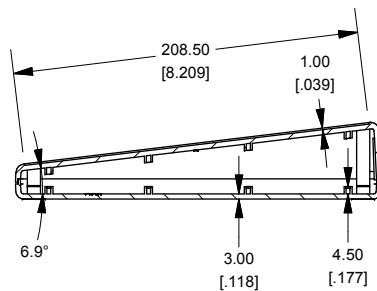
SECTION A-A Side View of Assembly
