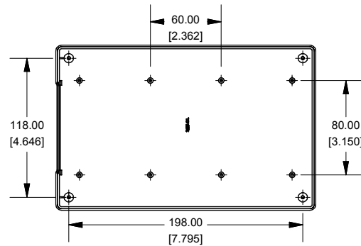
Bottom View Looking Inside Box
