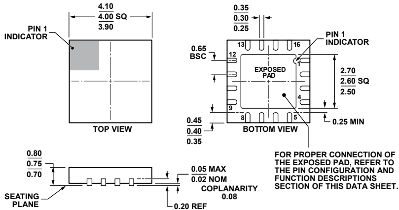
Figure 53. 16-Lead Lead Frame Chip Scale Package [LFCSF_WQ] 4 mm x 4 mm Body, Very Very Thin Quad (CP-16-17)
