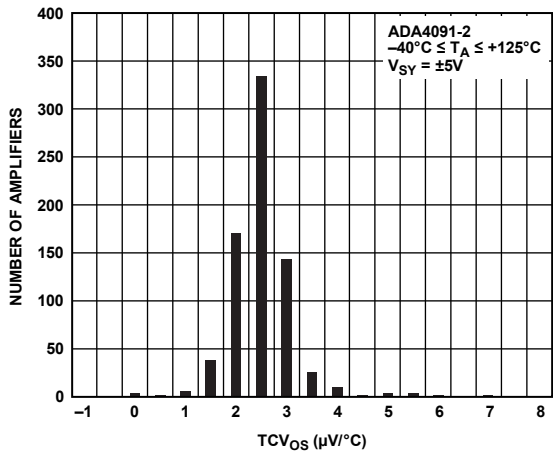
Figure 18. TCVos Distribution
