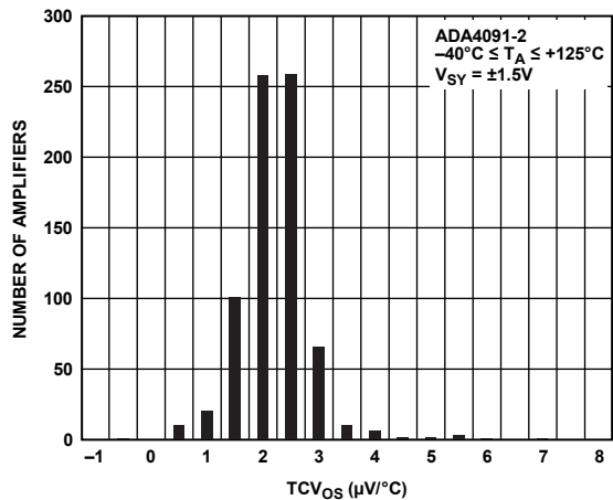
Figure 6. TCvos Distribution
