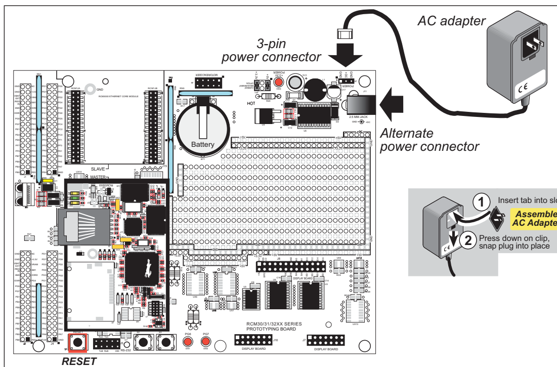
Figure 4. Power Supply Connections
