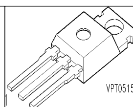
P-TO220-3-1
