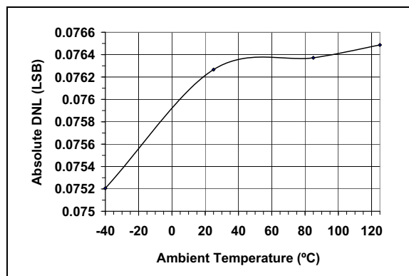
FIGURE 2-4: Absolute DNL vs. Temperature (MCP4921).
