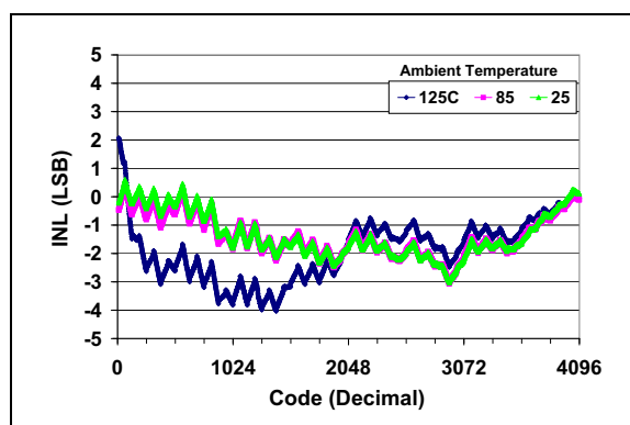
FIGURE 2-6: INL vs. Code and Temperature (MCP4921).
