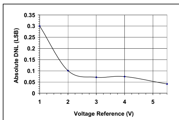
FIGURE 2-5: Absolute DNL vs. Voltage Reference (MCP4921).
