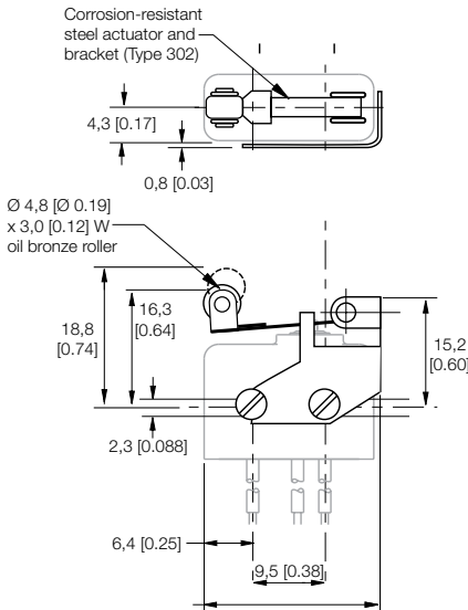
Figure 12. JM-5 Dimensions
