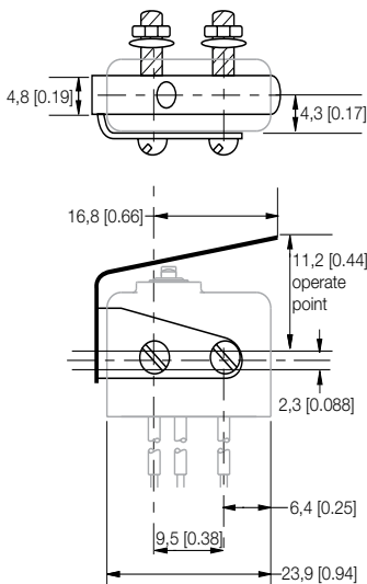
Figure 8. JE-17 Dimensions
