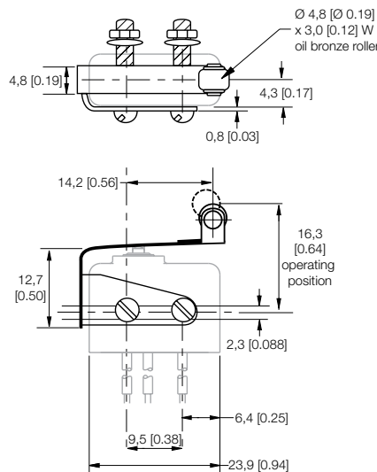
Figure 10. JE-22 Dimensions
