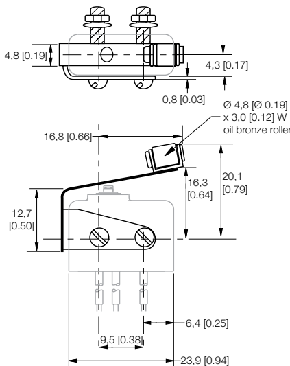
Figure 9. JE-21 Dimensions
