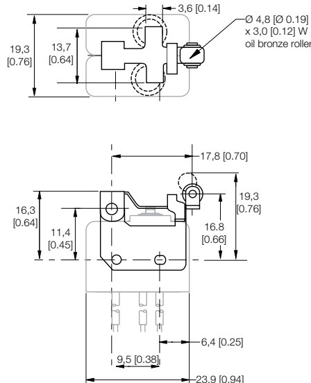
Figure 10. JE-22 Dimensions
