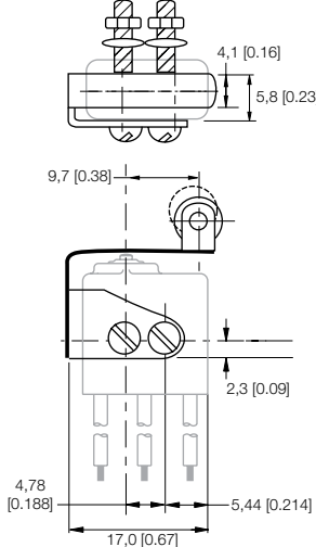
Figure 12. JM-5 Dimensions
