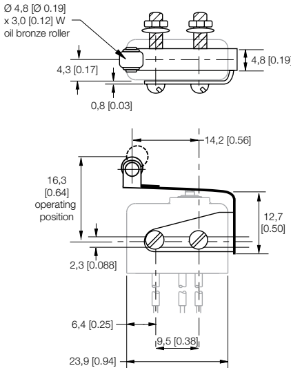
Figure 8. JE-17 Dimensions
