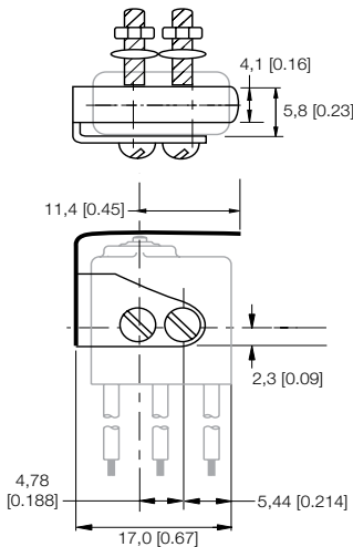
Figure 11. JM-1 Dimensions
