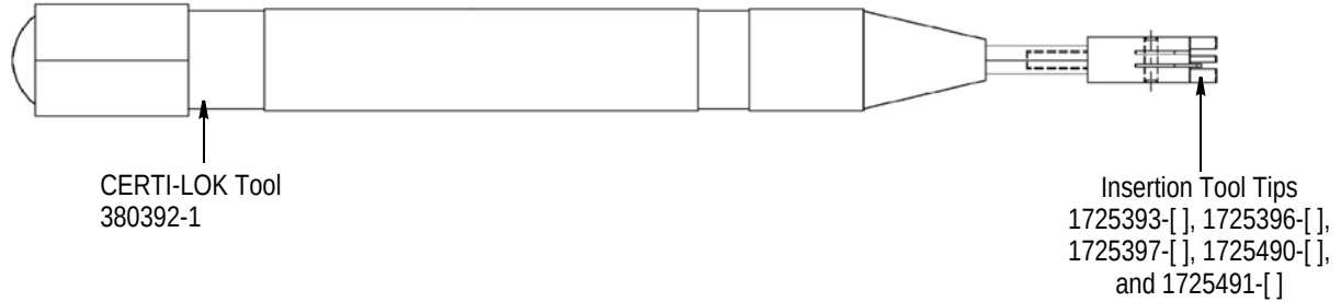
Repair Tool 1725385-[ ]
