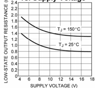
Low-State Output Resist. vs. Supply Voltage
