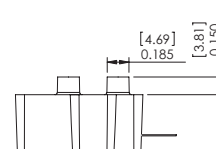
D- Two Ports Cut 0.150" Configuration
