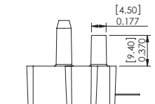
F- Port A Cut 0.370" Configuration
