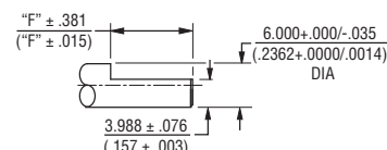
SHAFT TYPE "S" (USES BUSHING R)
