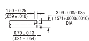
SHAFT TYPE "V" (USES BUSHING U)
