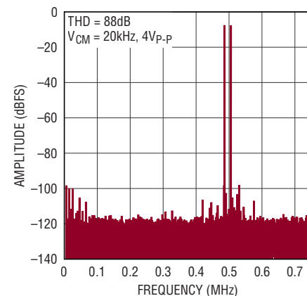
32k Point FFT, IMD, f_{\text{SAMPL}} = 1.5\text{Msps} , A_{\text{IN}}^+ = 490\text{kHz} , A_{\text{IN}}^- = 510\text{kHz}
