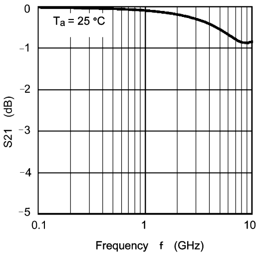
Fig. 9.5 S_{21} - f
