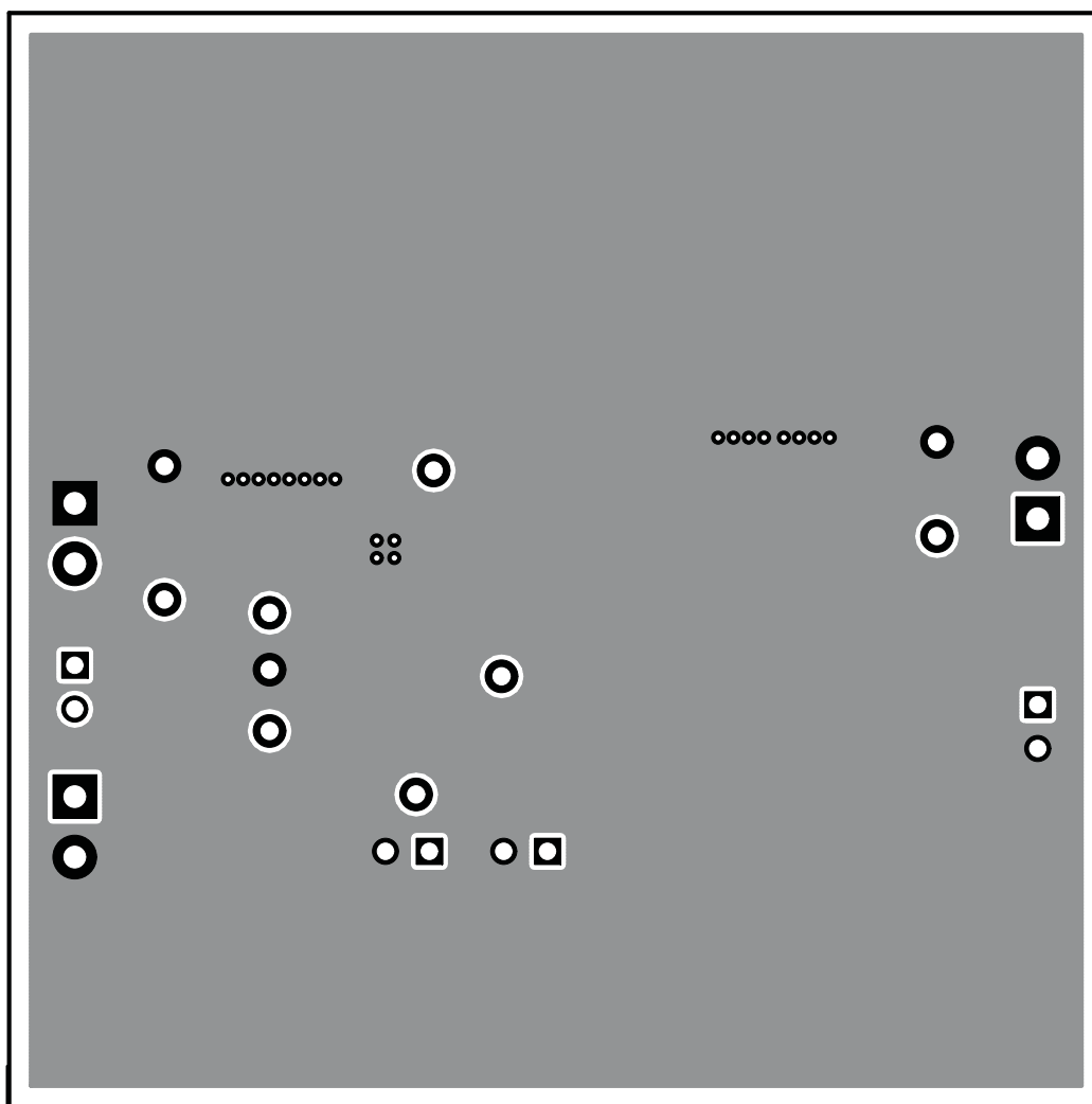
Figure 14. TPS54620EVM-374 Layout 3
