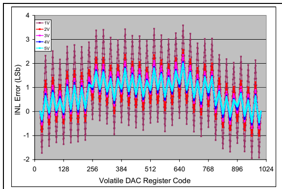
FIGURE 2-68: INL vs. Code (code = 25 to 1000) and V_{REF} (MCP4716). V_{DD} = 5\text{V} , V_{REF1}:V_{REF0} = 10 , G = 0 , V_{REF} = 1\text{V}, 2\text{V}, 3\text{V}, 4\text{V} , and 5\text{V} , \text{Temp} = +25^\circ\text{C} .
