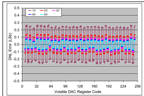
FIGURE 2-72: DNL vs. Code (code = 6 to 250) and V_{REF} (MCP4706). V_{DD} = 5\text{V} , V_{REF1}:V_{REF0} = 10 , G = 0 , V_{REF} = 1\text{V}, 2\text{V}, 3\text{V}, 4\text{V} , and 5\text{V} , \text{Temp} = +25^\circ\text{C} .
