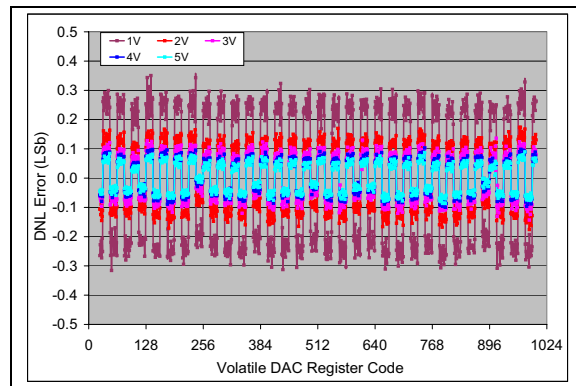
FIGURE 2-71: DNL vs. Code (code = 25 to 1000) and V_{REF} (MCP4716). V_{DD} = 5\text{V} , V_{REF1}:V_{REF0} = 10 , G = 0 , V_{REF} = 1\text{V}, 2\text{V}, 3\text{V}, 4\text{V} , and 5\text{V} , \text{Temp} = +25^\circ\text{C} .
