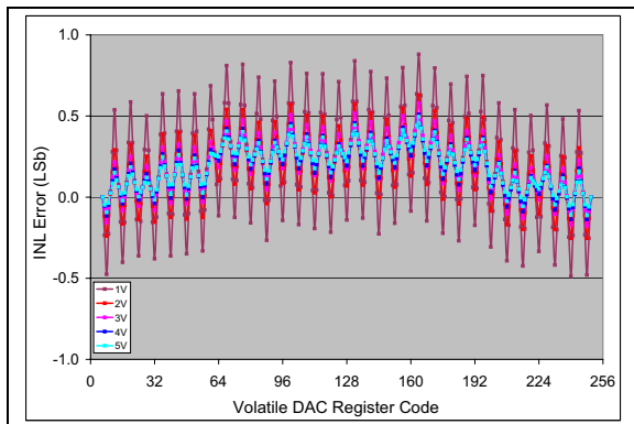
FIGURE 2-69: INL vs. Code (code = 6 to 250) and V_{REF} (MCP4706). V_{DD} = 5\text{V} , V_{REF1}:V_{REF0} = 10 , G = 0 , V_{REF} = 1\text{V}, 2\text{V}, 3\text{V}, 4\text{V} , and 5\text{V} , \text{Temp} = +25^\circ\text{C} .
