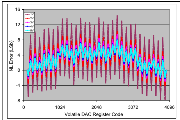
FIGURE 2-67: INL vs. Code (code = 100 to 4000) and V_{REF} (MCP4726). V_{DD} = 5\text{V} , V_{REF1}:V_{REF0} = 10 , G = 0 , V_{REF} = 1\text{V}, 2\text{V}, 3\text{V}, 4\text{V} , and 5\text{V} , \text{Temp} = +25^\circ\text{C} .
