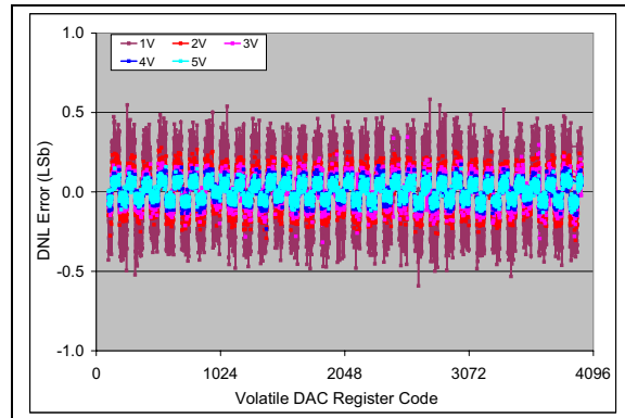
FIGURE 2-70: DNL vs. Code (code = 100 to 4000) and V_{REF} (MCP4726). V_{DD} = 5\text{V} , V_{REF1}:V_{REF0} = 10 , G = 0 , V_{REF} = 1\text{V}, 2\text{V}, 3\text{V}, 4\text{V} , and 5\text{V} , \text{Temp} = +25^\circ\text{C} .
