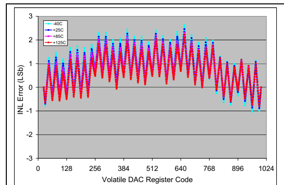
FIGURE 2-5: INL vs. Code (code = 25 to 1000) and Temperature (MCP4716). V_{DD} = 2.7\text{V} , V_{REF1}:V_{REF0} = 00 .
