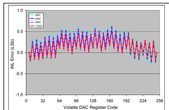
FIGURE 2-6: INL vs. Code (code = 6 to 250) and Temperature (MCP4706). V_{DD} = 2.7\text{V} , V_{REF1}:V_{REF0} = 00 .
