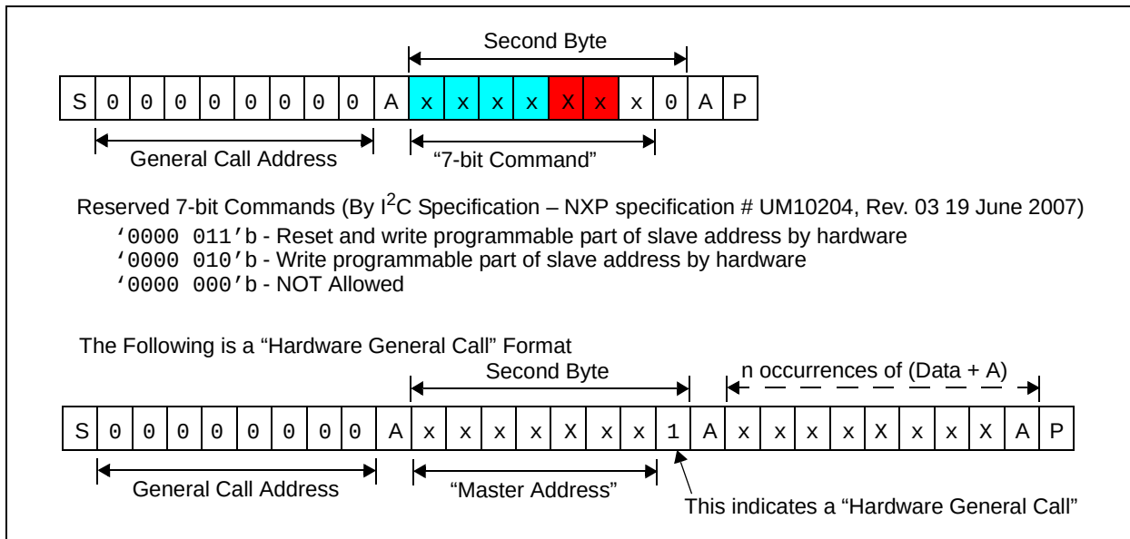
FIGURE 5-11: General Call Formats.
