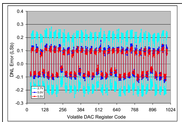
FIGURE 2-59: DNL vs. Code (code = 25 to 1024) and V_{DD} (2.7V, 5V, 5.5V) (MCP4716). V_{REF1}:V_{REF0} = 10 , G = 1 , V_{REF} = V_{DD}/2 , \text{Temp} = +25^\circ\text{C} .
