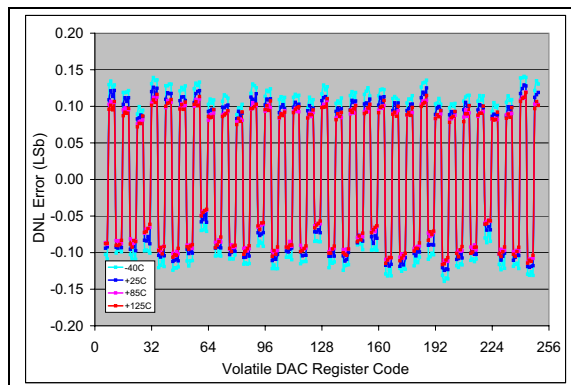
FIGURE 2-12: DNL vs. Code (code = 6 to 250) and Temperature (MCP4706).
