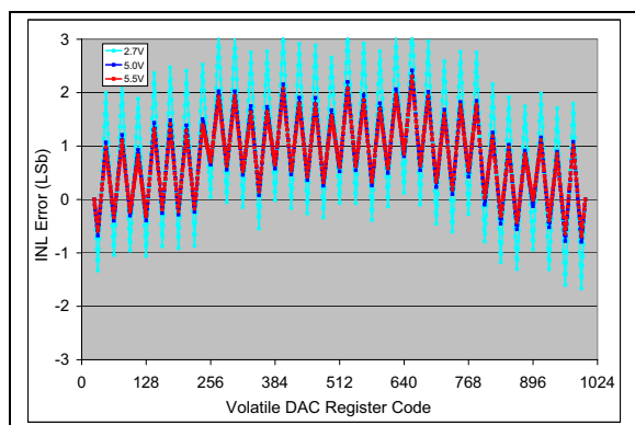
FIGURE 2-56: INL vs. Code (code = 25 to 1024) and V_{DD} (2.7V, 5V, 5.5V) (MCP4716). V_{REF1}:V_{REF0} = 10 , G = 1 , V_{REF} = V_{DD}/2 , \text{Temp} = +25^\circ\text{C} .
