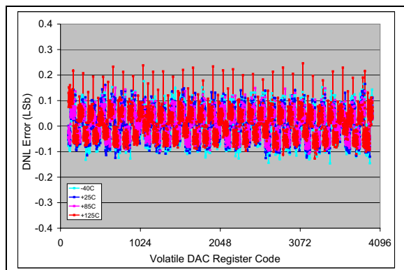
FIGURE 2-7: DNL vs. Code (code = 100 to 4000) and Temperature (MCP4726).
