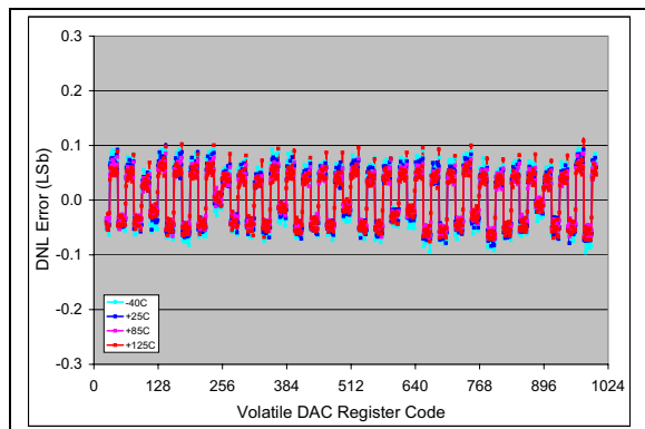
FIGURE 2-8: DNL vs. Code (code = 25 to 1000) and Temperature (MCP4716).
