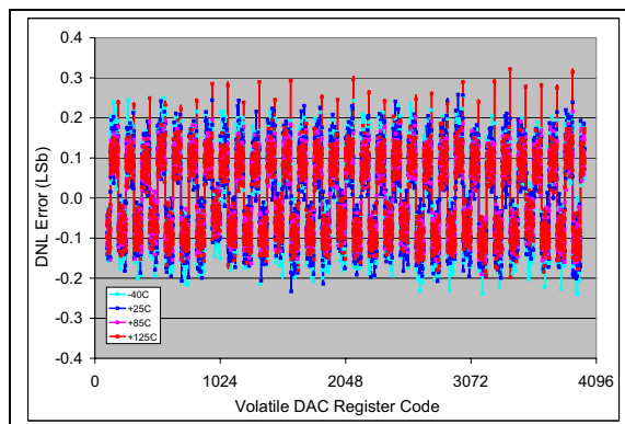
FIGURE 2-10: DNL vs. Code (code = 100 to 4000) and Temperature (MCP4726).
