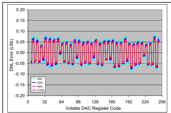
FIGURE 2-9: DNL vs. Code (code = 6 to 250) and Temperature (MCP4706).
