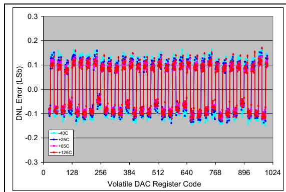
FIGURE 2-11: DNL vs. Code (code = 25 to 1000) and Temperature (MCP4716).
