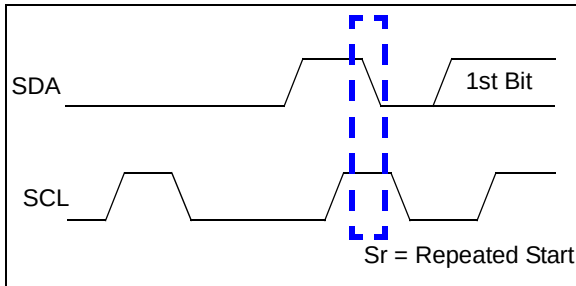
FIGURE 5-5: Repeat Start Condition Waveform.
