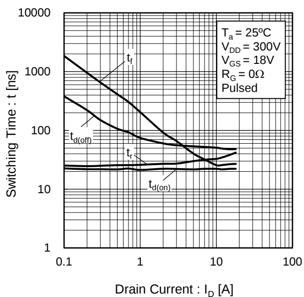
Fig.17 Switching Characteristics
