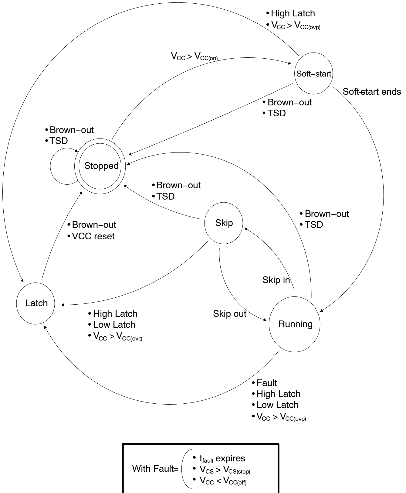
Figure 53. Controller Operation State Diagram (Latched Protection)
