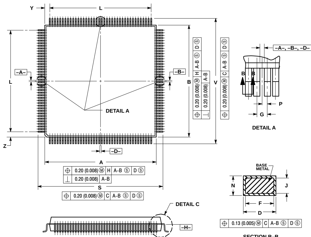
SECTION B-B
