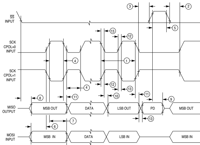
Figure A-18 QSPI Timing — Slave, CPHA = 0
