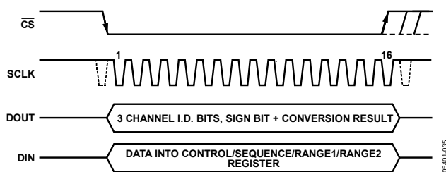
Figure 48. Normal Mode
