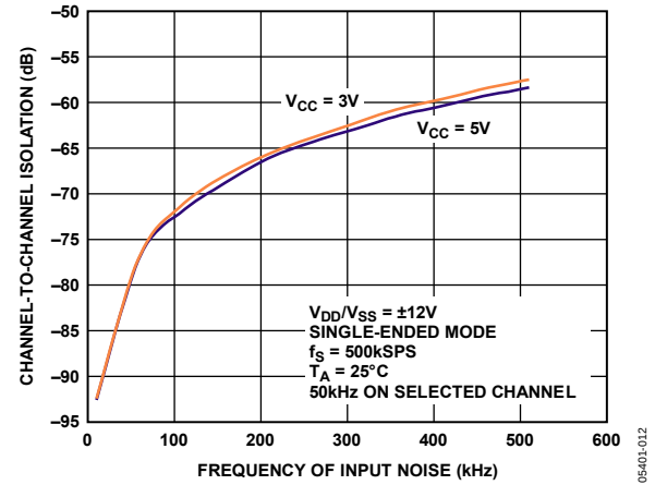
Figure 14. Channel-to-Channel Isolation
