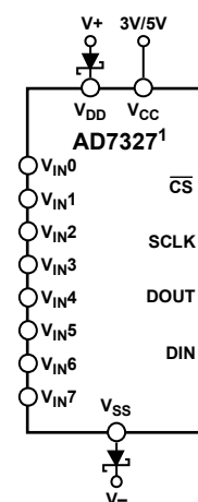
1 ADDITIONAL PINS OMITTED FOR CLARITY.
