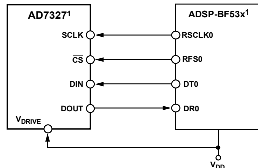
Figure 55. Interfacing the AD7327 to the ADSP-BF53x
