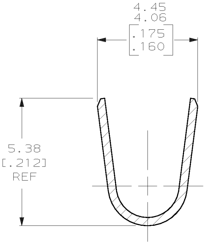
SECTION C-C SCALE 10:1
