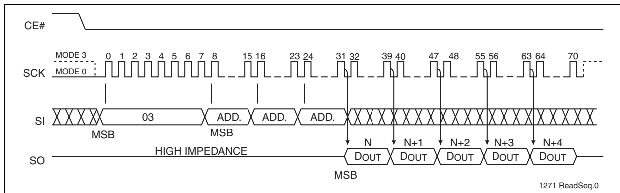
FIGURE 4-3: READ SEQUENCE
