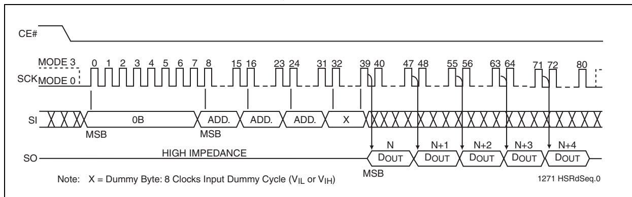
FIGURE 4-4: HIGH-SPEED-READ SEQUENCE
