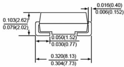
SMA/DO-214AB
