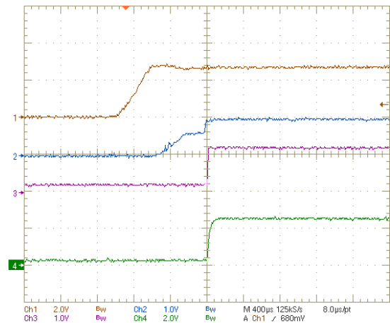
FIGURE 15. 4-CHANNEL DEFAULT START-UP @ FULL LOAD CH1: VODCD1 (2V/DIV), CH2: VODCD2 (1V/DIV), CH3: VOLD01 (1V/DIV), CH4: VOLD02 (2V/DIV)
