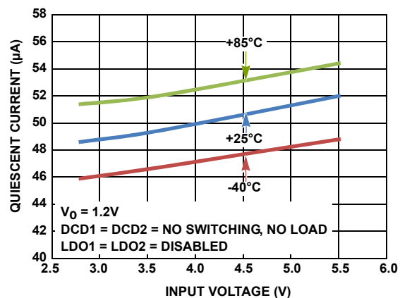
FIGURE 21. QUIESCENT CURRENT vs INPUT VOLTAGE
