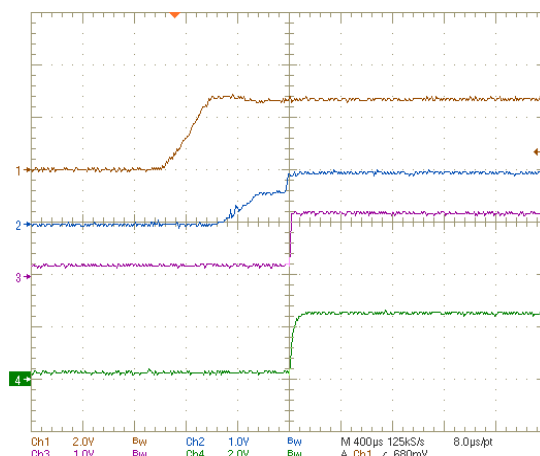
FIGURE 15. 4-CHANNEL DEFAULT START-UP @ FULL LOAD CH1: VODCD1 (2V/DIV), CH2: VODCD2 (1V/DIV), CH3: VOLD01 (1V/DIV), CH4: VOLD02 (2V/DIV)
