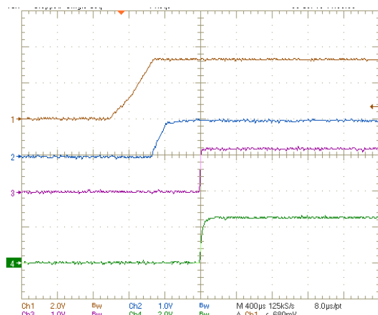
FIGURE 14. 4-CHANNEL DEFAULT START-UP @ NO LOAD CH1: VODCD1 (2V/DIV), CH2: VODCD2 (1V/DIV), CH3: VOLD01 (1V/DIV), CH4: VOLD02 (2V/DIV)
