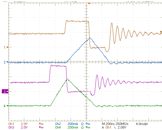
FIGURE 10. INDUCTOR CURRENT RIPPLE ( V_{IN} = 3.6V , PFM, TIME SCALE = 200ns) CH1: SW1 (2V/DIV), CH2: IL1 (200mA/DIV), CH3: SW2 (2V/DIV), CH4: IL2 (200mA/DIV)
