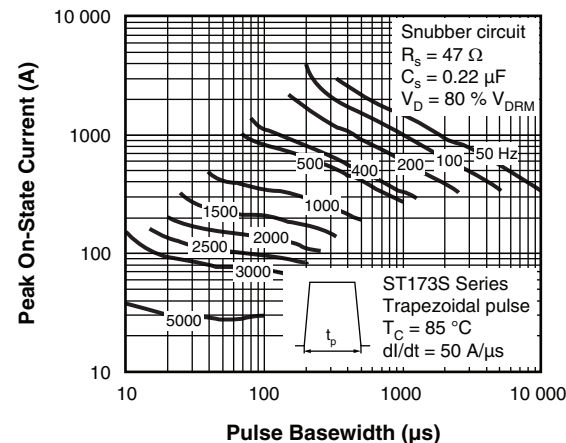
Fig. 12 - Frequency Characteristics
