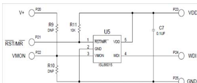
FIGURE 21. ISL88015EVAL1Z
