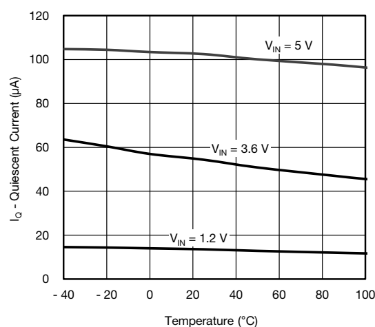
Figure 8 - Quiescent Current vs. Temperature
