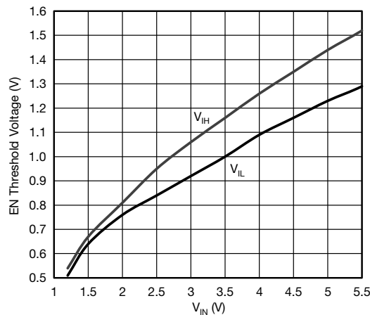
Figure 19 - EN Threshold Voltage vs. Input Voltage
