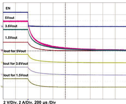
Figure 30 - Typical Fall Time C_{OUT} = 100 \mu F , C_{IN} = 4.7 \mu F , I_{OUT} = 1.5 A
