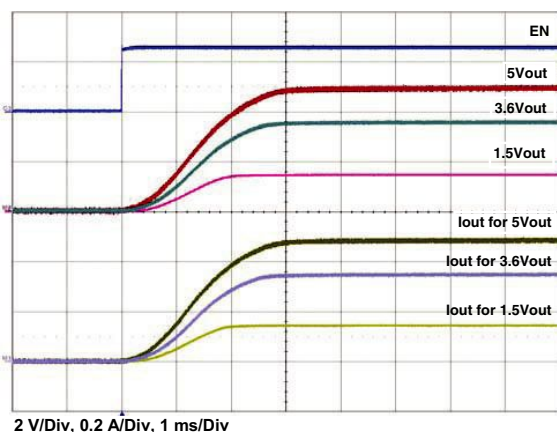
Figure 28 - Typical Turn-on Delay, Rise Time C_{OUT} = 100 \mu F , C_{IN} = 4.7 \mu F , R_{OUT} = 10 \Omega
