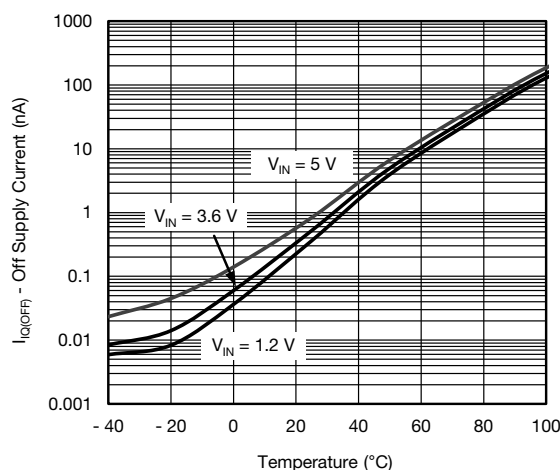
Figure 9 - Off Supply Current vs. Temperature
