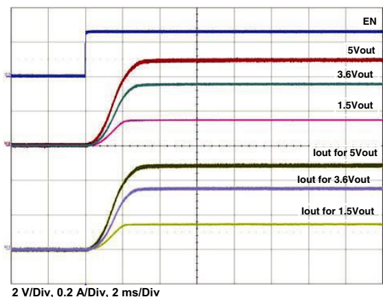
Figure 26 - Typical Turn-on Delay, Rise Time C_{OUT} = 200 \mu F , C_{IN} = 4.7 \mu F , R_{OUT} = 10 \Omega
