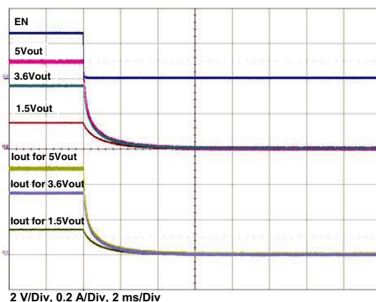
Figure 31 - Typical Turn-on Delay, Fall Time C_{OUT} = 100 \mu F , C_{IN} = 4.7 \mu F , R_{OUT} = 10 \Omega
