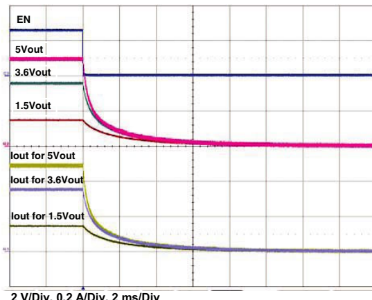
Figure 29 - Typical Fall Time C_{OUT} = 200 \mu F , C_{IN} = 4.7 \mu F , R_{OUT} = 10 \Omega
