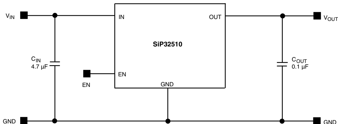
Figure 1 - SiP32510 Typical Application Circuit
