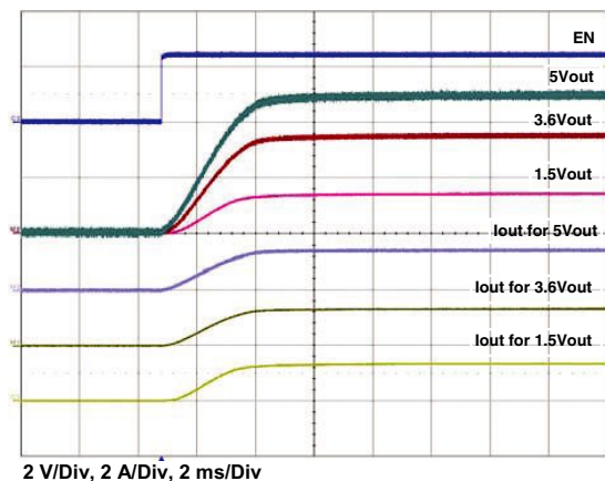
Figure 20 - Typical Turn-on Delay, Rise Time C_{OUT} = 0.1 \mu F , C_{IN} = 4.7 \mu F , I_{OUT} = 1.5 A
