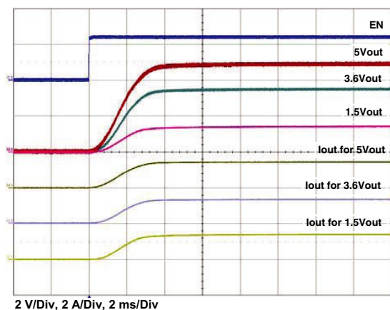
Figure 22 - Typical Turn-on Delay, Rise Time C_{OUT} = 200 \mu F , C_{IN} = 4.7 \mu F , I_{OUT} = 1.5 A
