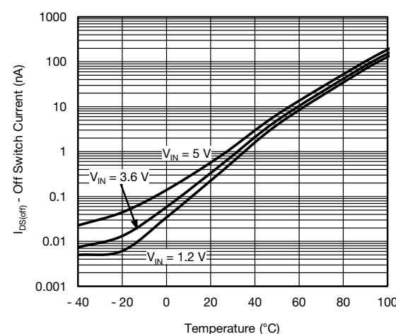
Figure 10 - Off Switch Current vs. Temperature
