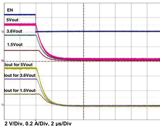
Figure 24 - Typical Fall Time C_{OUT} = 0.1 \mu F , C_{IN} = 4.7 \mu F , R_{OUT} = 10 \Omega
