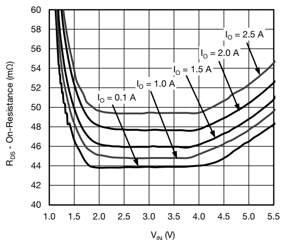
Figure 11 - On-Resistance vs. Input Voltage
