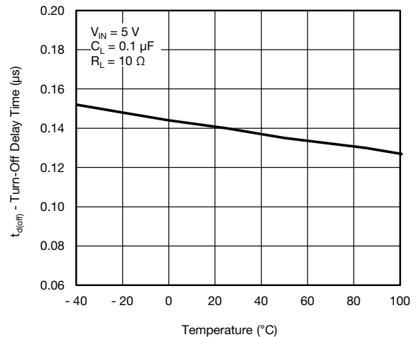
Figure 18 - Turn-Off Delay Time vs. Temperature
