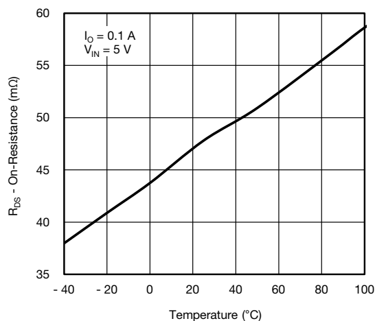
Figure 13 - On-Resistance vs. Temperature
