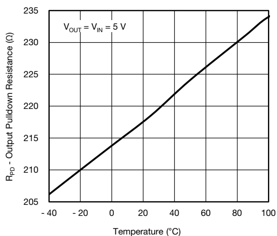
Figure 14 - Output Pulldown Resistance vs. Temperature
