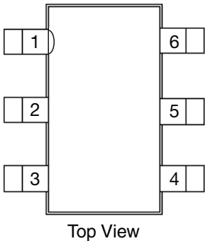
Figure 3 - TSOT23-6 Package
