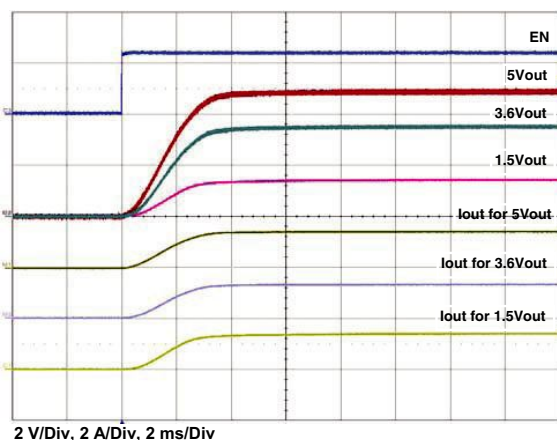
Figure 27 - Typical Turn-on Delay, Rise Time C_{OUT} = 100 \mu F , C_{IN} = 4.7 \mu F , I_{OUT} = 1.5 A
