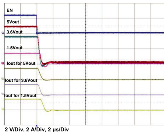
Figure 23 - Typical Fall Time C_{OUT} = 0.1 \mu F , C_{IN} = 4.7 \mu F , I_{OUT} = 1.5 A
