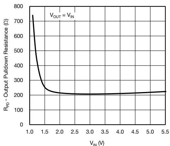
Figure 12 - Output Pulldown Resistance vs. Input Voltage
