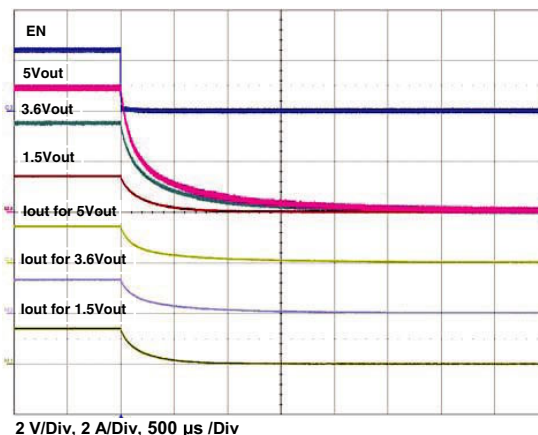
Figure 25 - Typical Fall Time C_{OUT} = 200 \mu F , C_{IN} = 4.7 \mu F , I_{OUT} = 1.5 A
