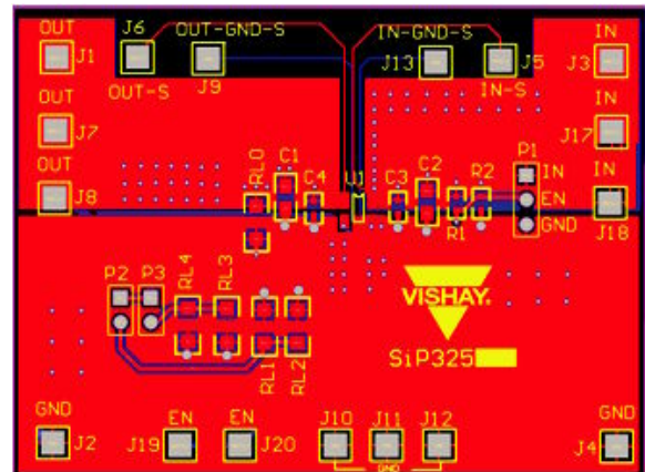
Figure 32 - Evaluation Board Layout for TSOT23-6L
