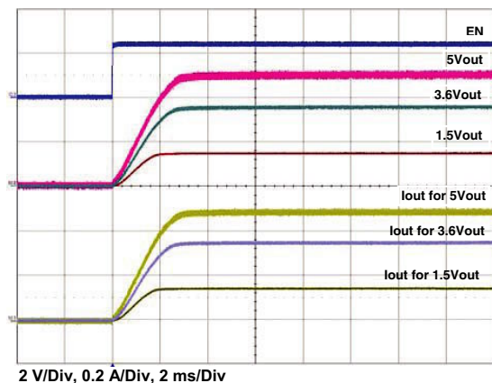
Figure 21 - Typical Turn-on Delay, Rise Time C_{OUT} = 0.1 \mu F , C_{IN} = 4.7 \mu F , R_{OUT} = 10 \Omega
